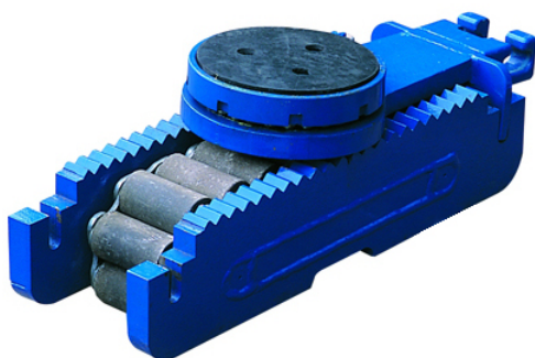
VP Rubber Top Swivel shown fitted to a VB Roller Skate
